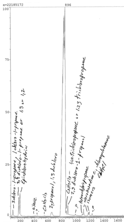
Figure 2. Sample total ion chromatogram from total GC/MS. Note that Fenton reaction--presumably like other oxidants used in ISCO—degrades TCP to a complex mixture of oxygenated and relatively polar products.
