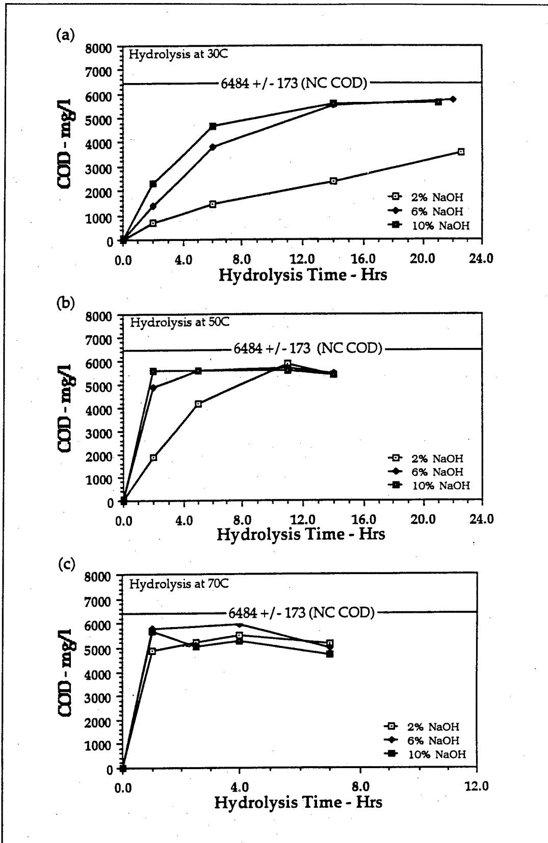
Figure 35. Hydrolysate COD following hydrolysis at (a) 30 °C, (b) 50 °C, and (c) 70 °C.
