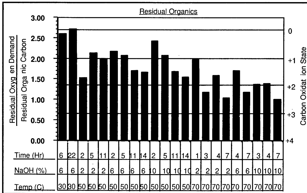
Figure 43. ROD/TOC (residual) ratios versus the hydrolysis conditions.
