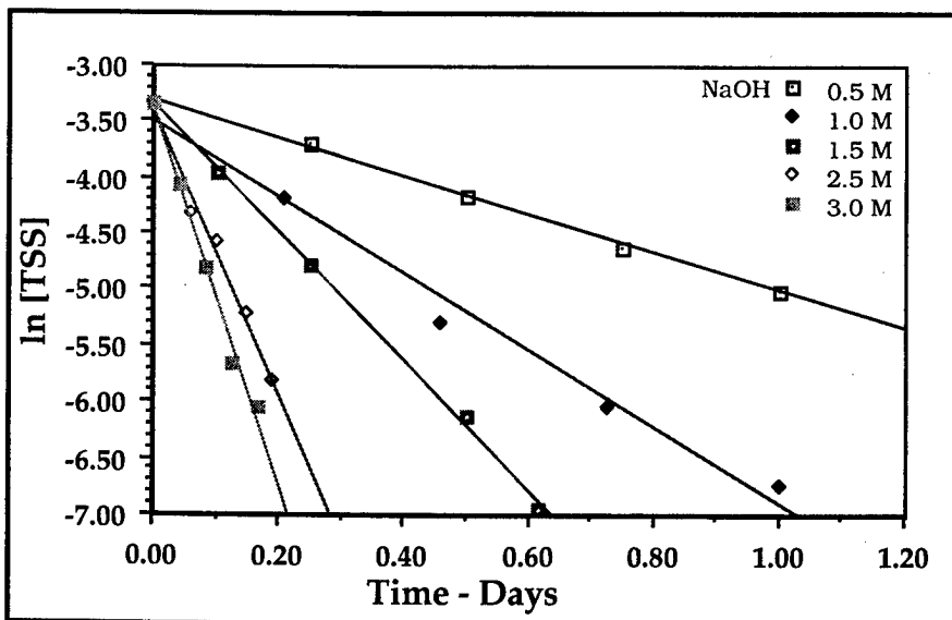
Figure 21. \ln [TSS] versus time, as a function of caustic dose.
