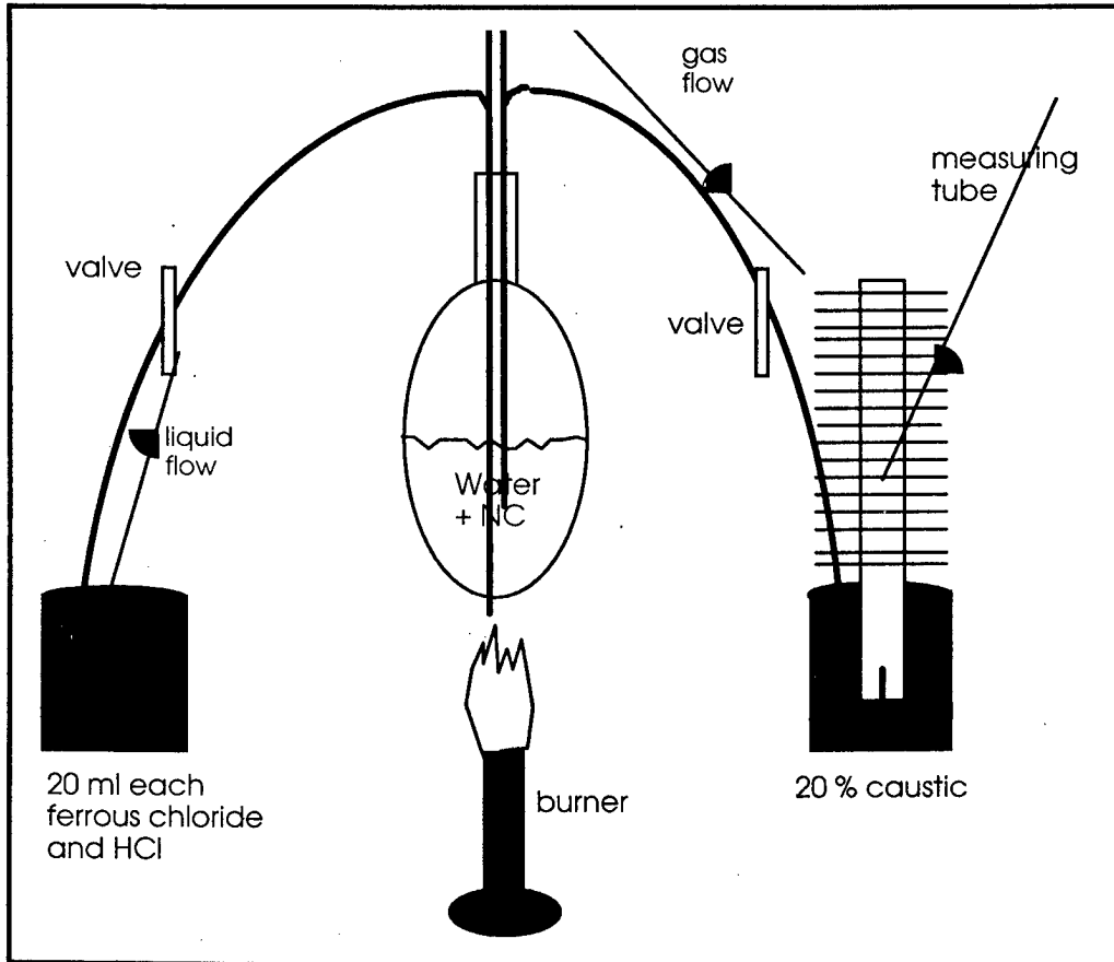
Figure 4. Schultz-Tiemann test apparatus.
