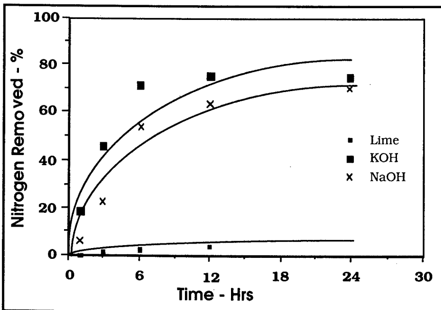
Figure 13. Nitrogen yield relative to caustic species.
