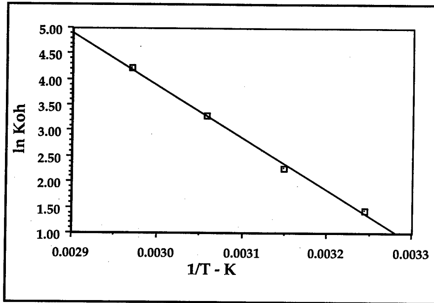
Figure 24. In KOH versus 1/T (°K).
