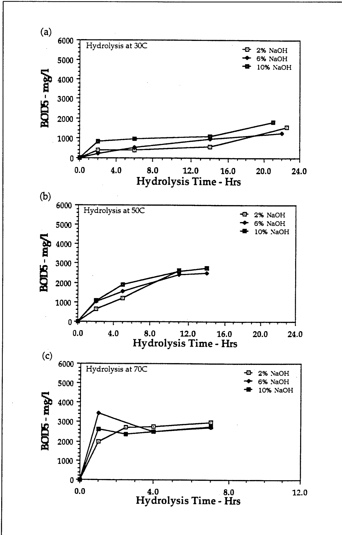
Figure 39. Hydrolysate BOD5 following hydrolysis at (a) 30°C, (b) 50°C, and (c) 70°C.
