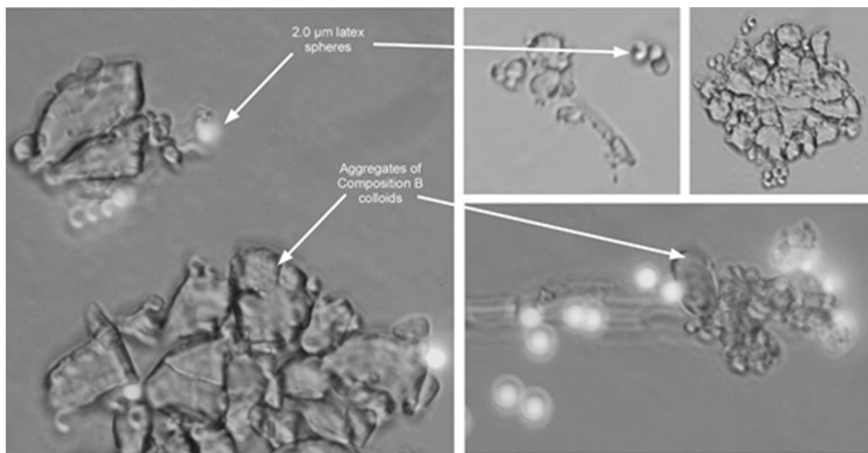
Figure 1-3. Photomicrographs of colloidal Composition B in water. Spherical particles are 2.0 \mu\text{m} fluorescent latex beads.
