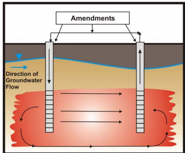
Figure 5.3 Schematic of a Horizontal Recirculation System
